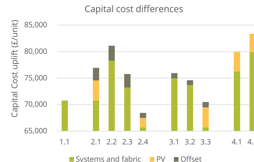
Figure 5.1.8: An example of the capital costs differences for the Terrace house
