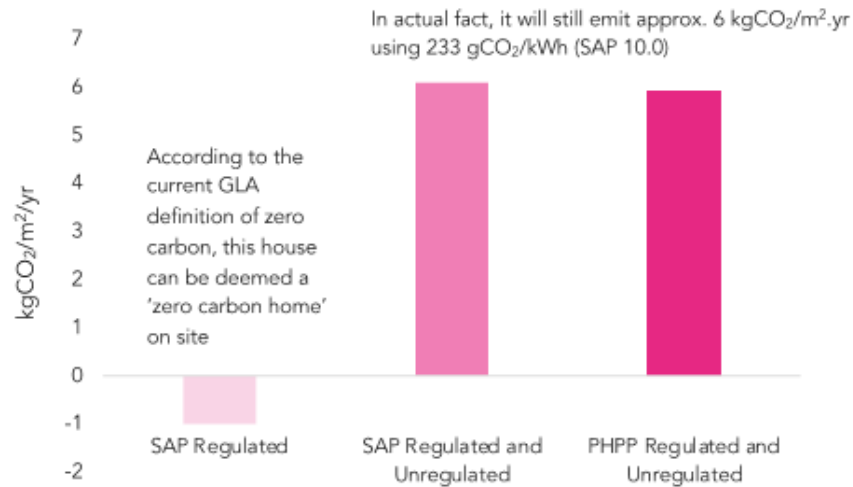
Figure 3.5.1: Carbon emission reductions at various carbon factors – a home with a heat pump
