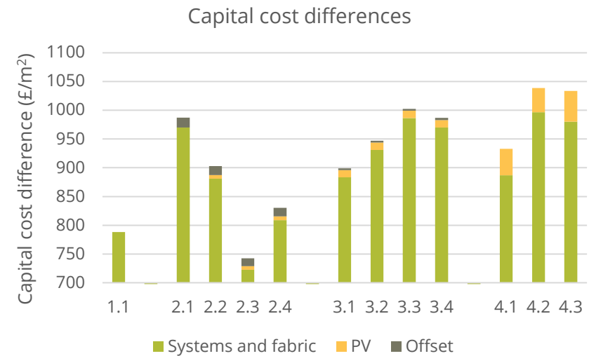
Figure 5.4.5 Difference in Capital Cost/m 2
