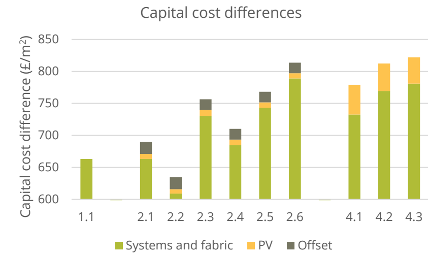
Figure 5.5.4 Difference in Capital Cost/ unit
