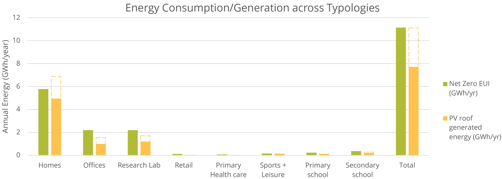
Figure 6.1.1 Energy consumption/generation across the Garden Village typologies
