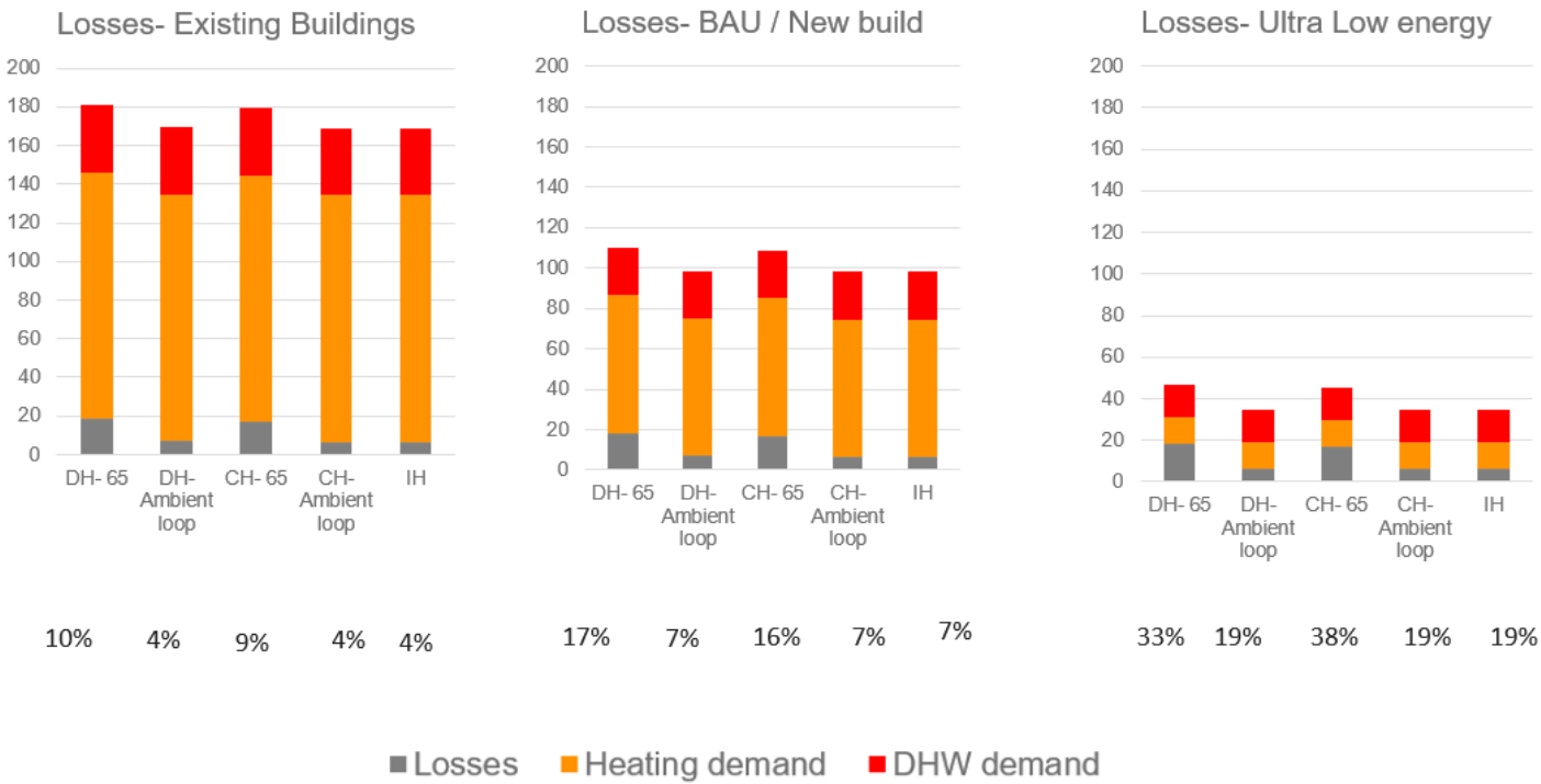
Figure 9.1.1: Losses in district, communal and individual heating systems
